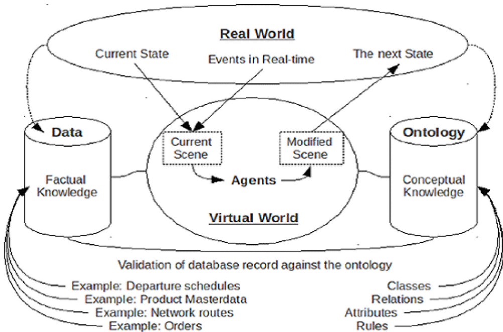
Figure 1. Conceptual architecture of multi-agent solution for LEGO
